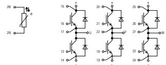
sixpack with NTC
