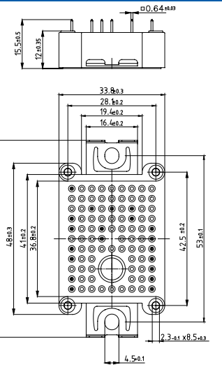
- Pinpositions typ. \pm 0.4
