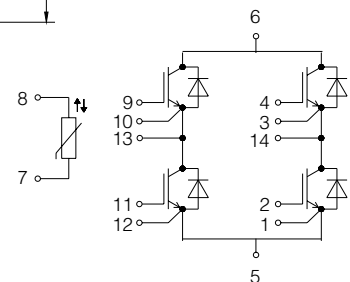
fourpack with NTC
