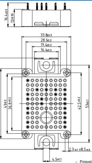
- Pinpositions typ. \pm 0.4
