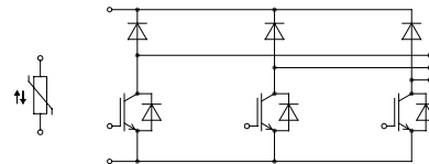
FD chopper with NTC
