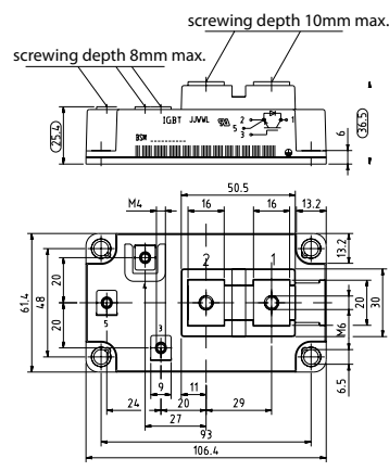
Single Switch 62, collector sense
