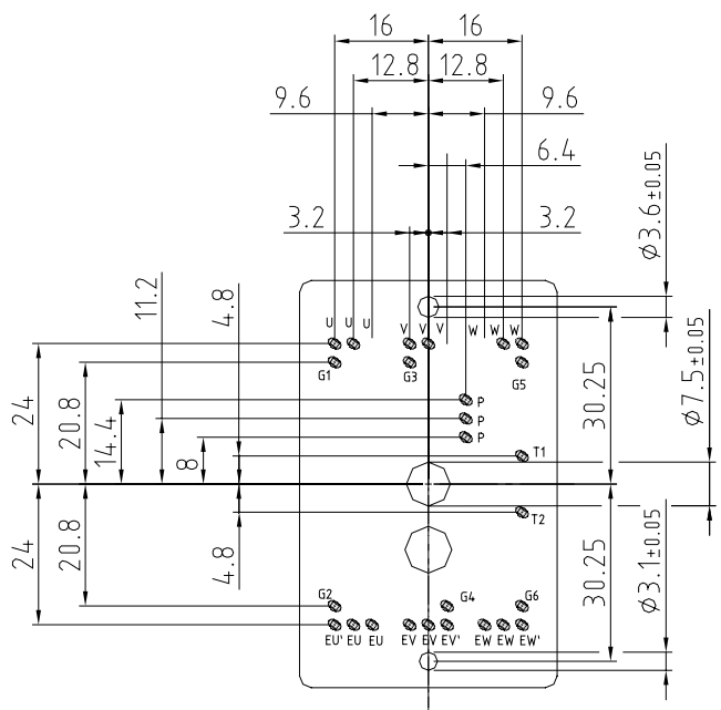
PCB hole pattern
