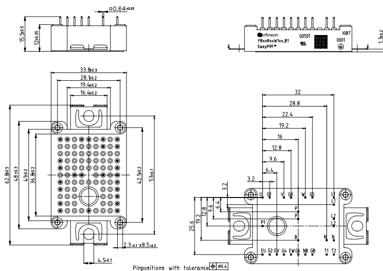
Pinpositions with tolerance \pm 0.4
