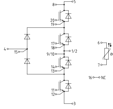
3-level one-phase NPC1 topology with NTC
