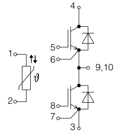
dual modules with NTC
