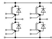
fourpack without NTC
