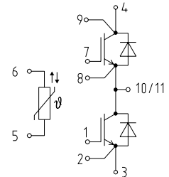
dual modules with NTC
