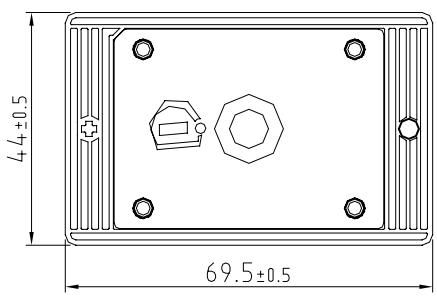
top view of pressure part
