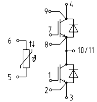
3-level one-phase NPC1 topology with NTC
