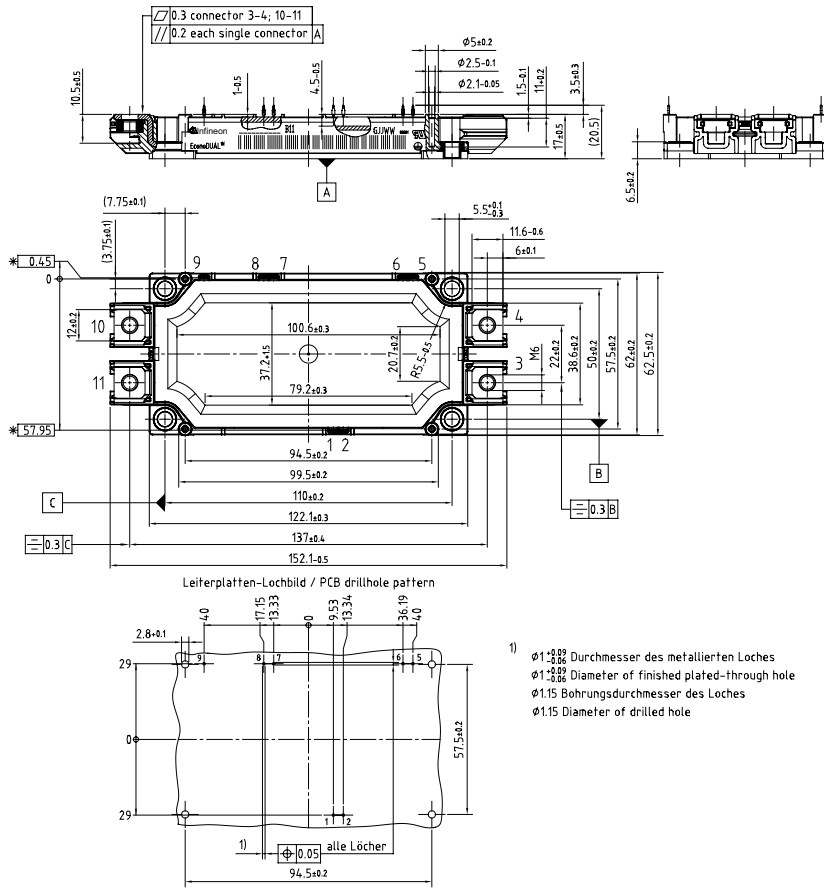
dual modules with NTC
