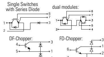
Single Switch 62, collector sense
